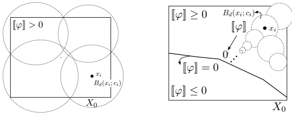
Figure 2: Robust testing terminates on robustly correct systems (left), but not necessarily on non-robust systems where the robustness vanishes gradually (right).
